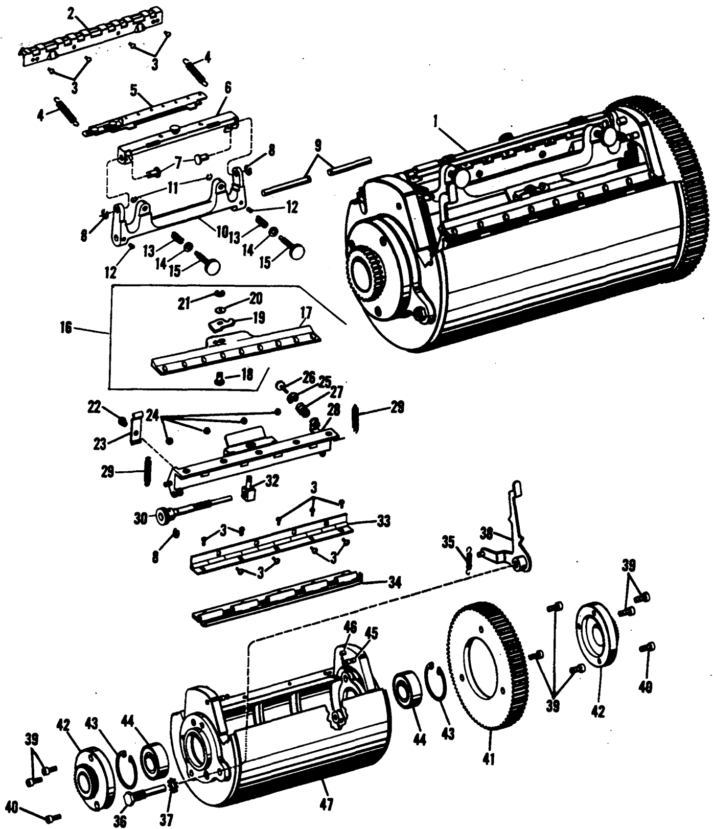
FIGURE 20B MODEL 8805/8820 Master Cylinder 10" x 15" Plates
