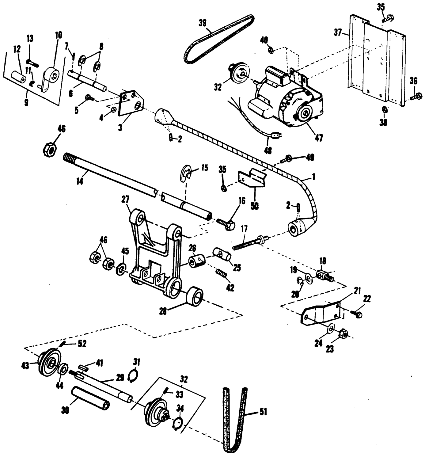
FIGURE 52 MODEL 8805/8820 Machine Speed Control
