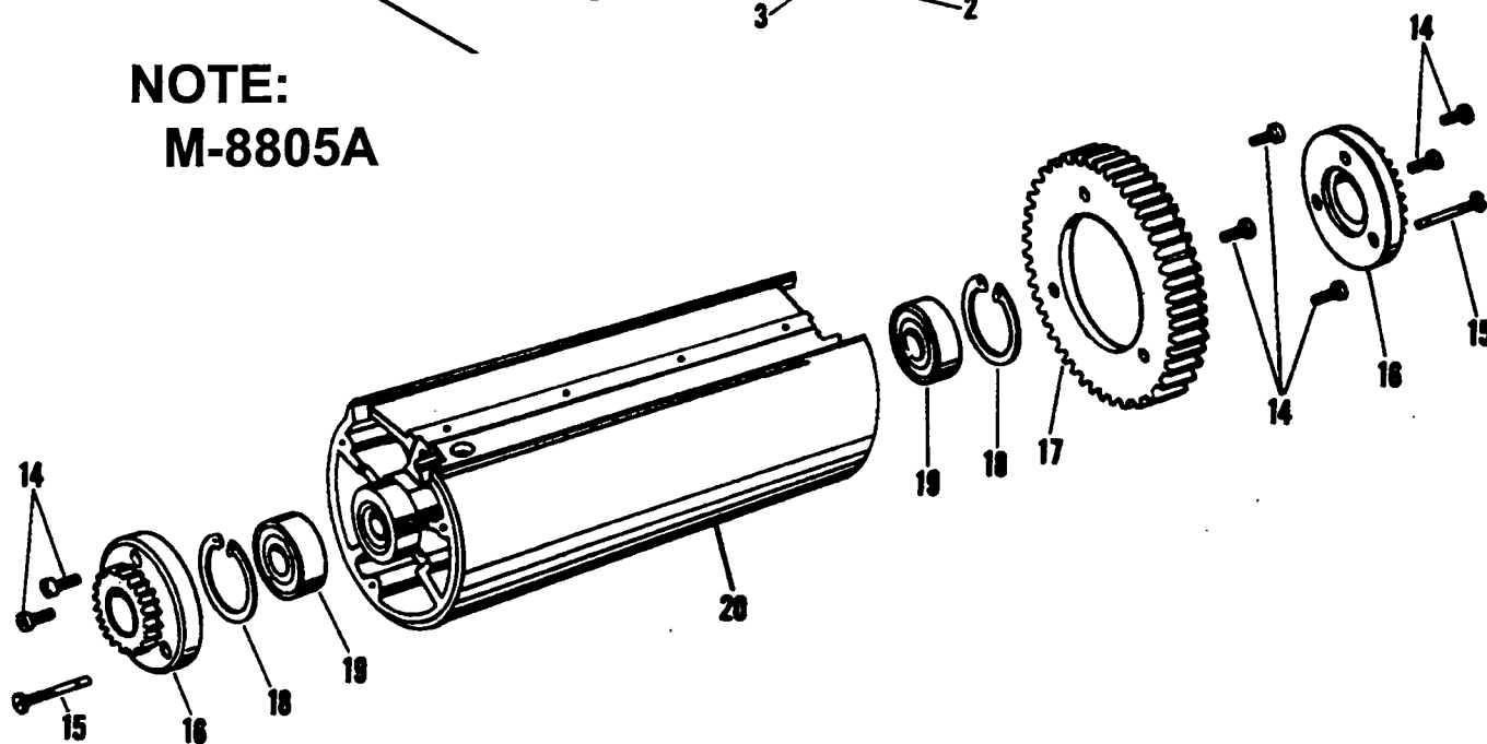
FIGURE 20A MODEL 8805/8820 Aluminum Master Cylinder
