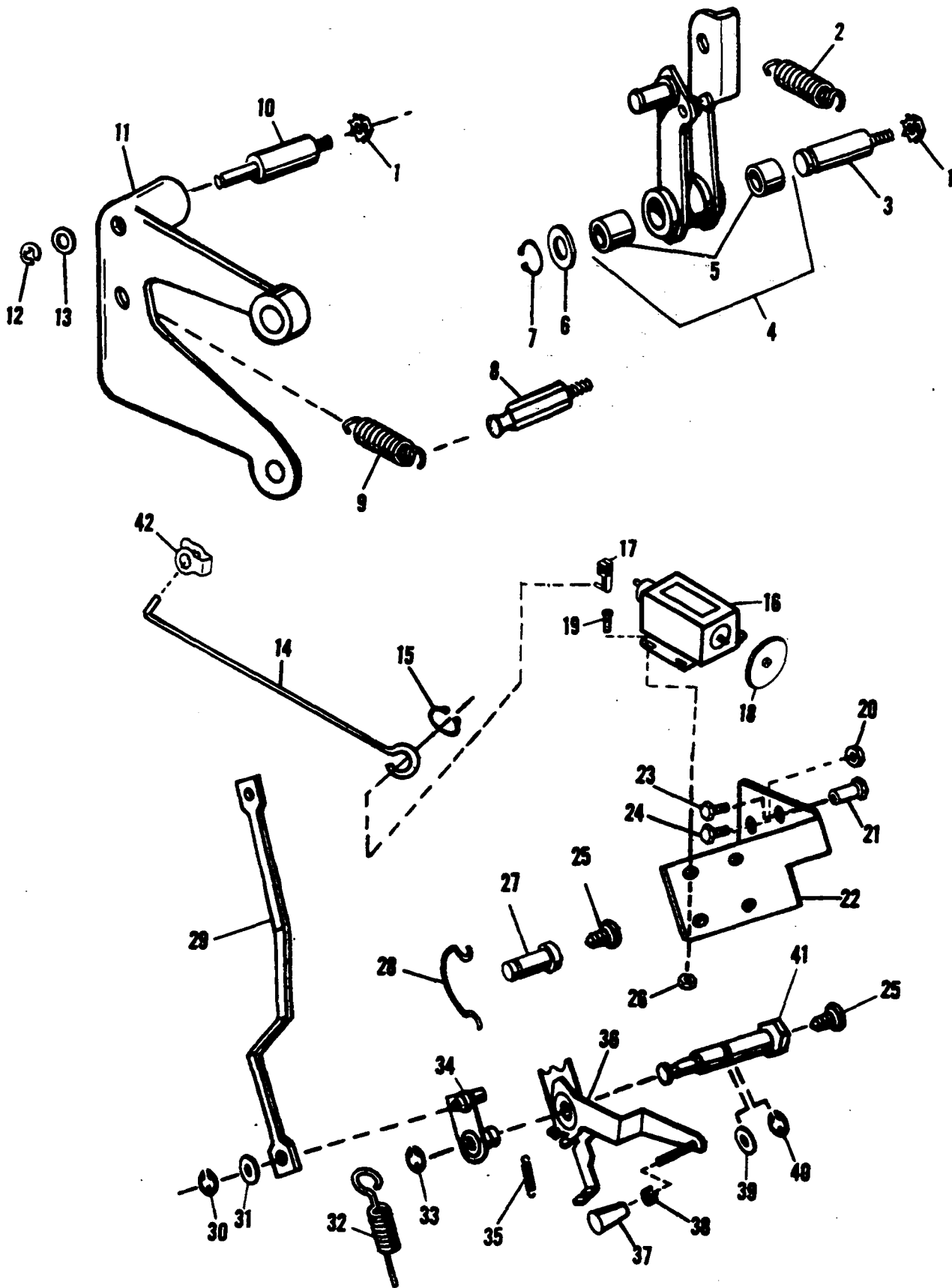
FIGURE 31 MODEL 8805/8820 Counter and Feed Levers
