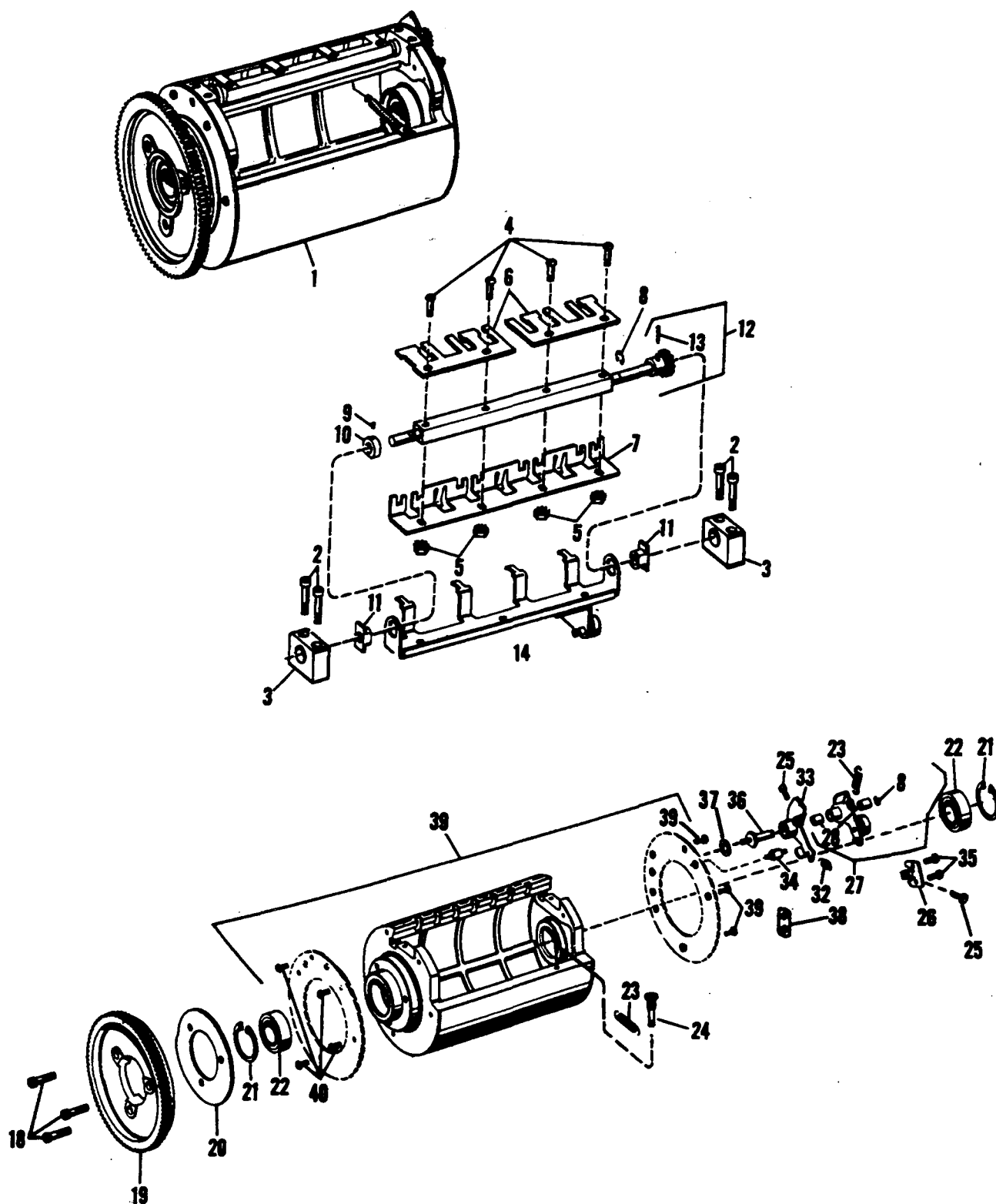
FIGURE 28 MODEL 8805/8820 Impression Cylinder Assembly
