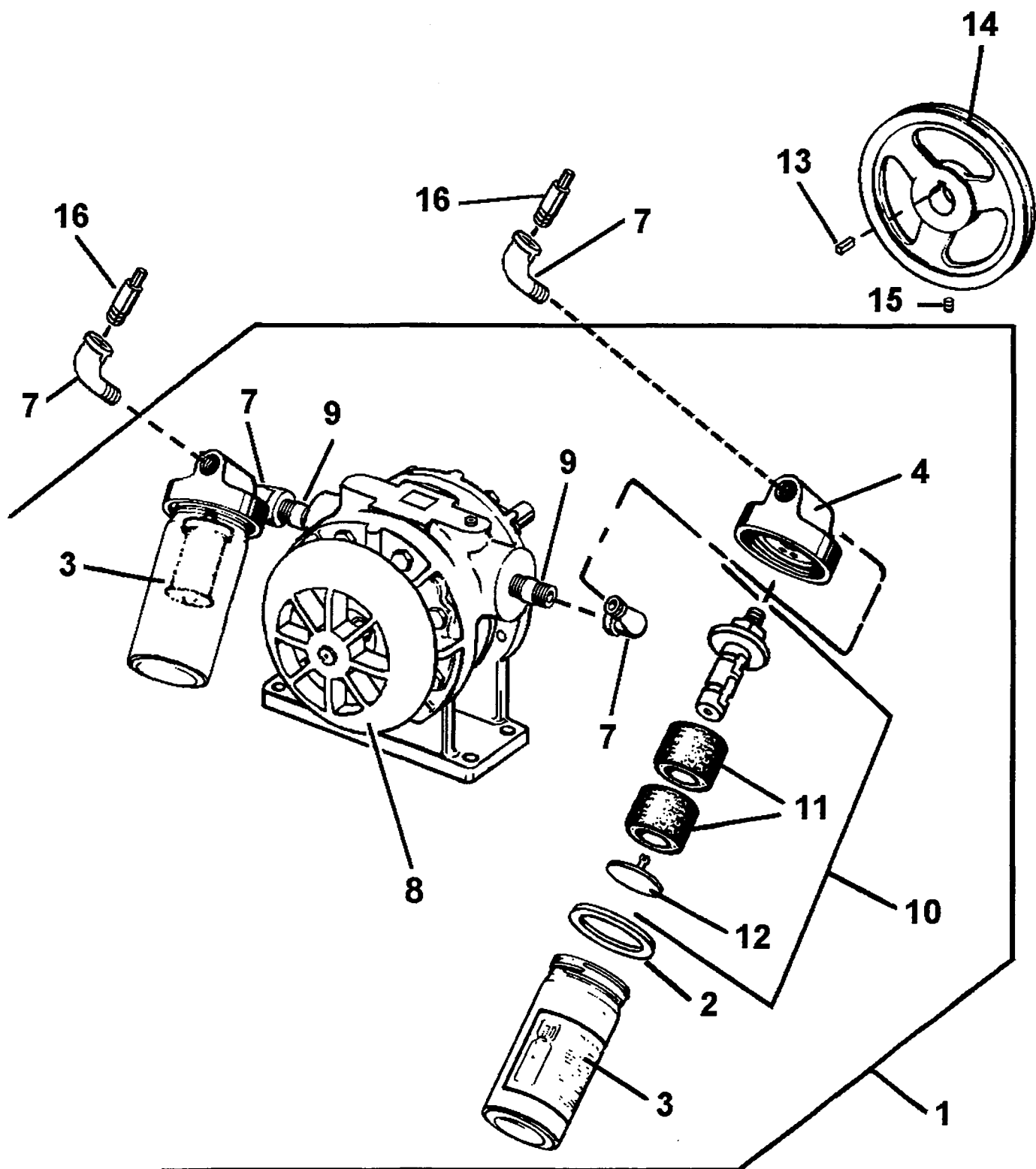
FIGURE 54A MODEL 8805/8820 Compressor Assembly (New Design)
