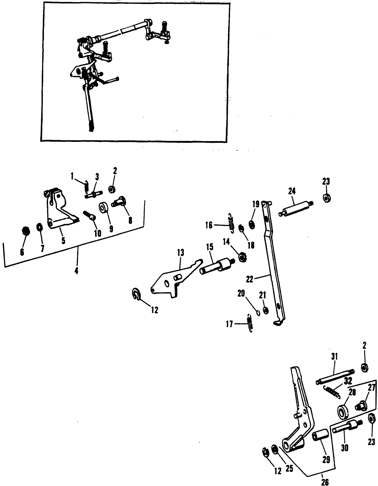
FIGURE 24 MODEL 8805/8820 Master Cylinder Lever Assemblies
