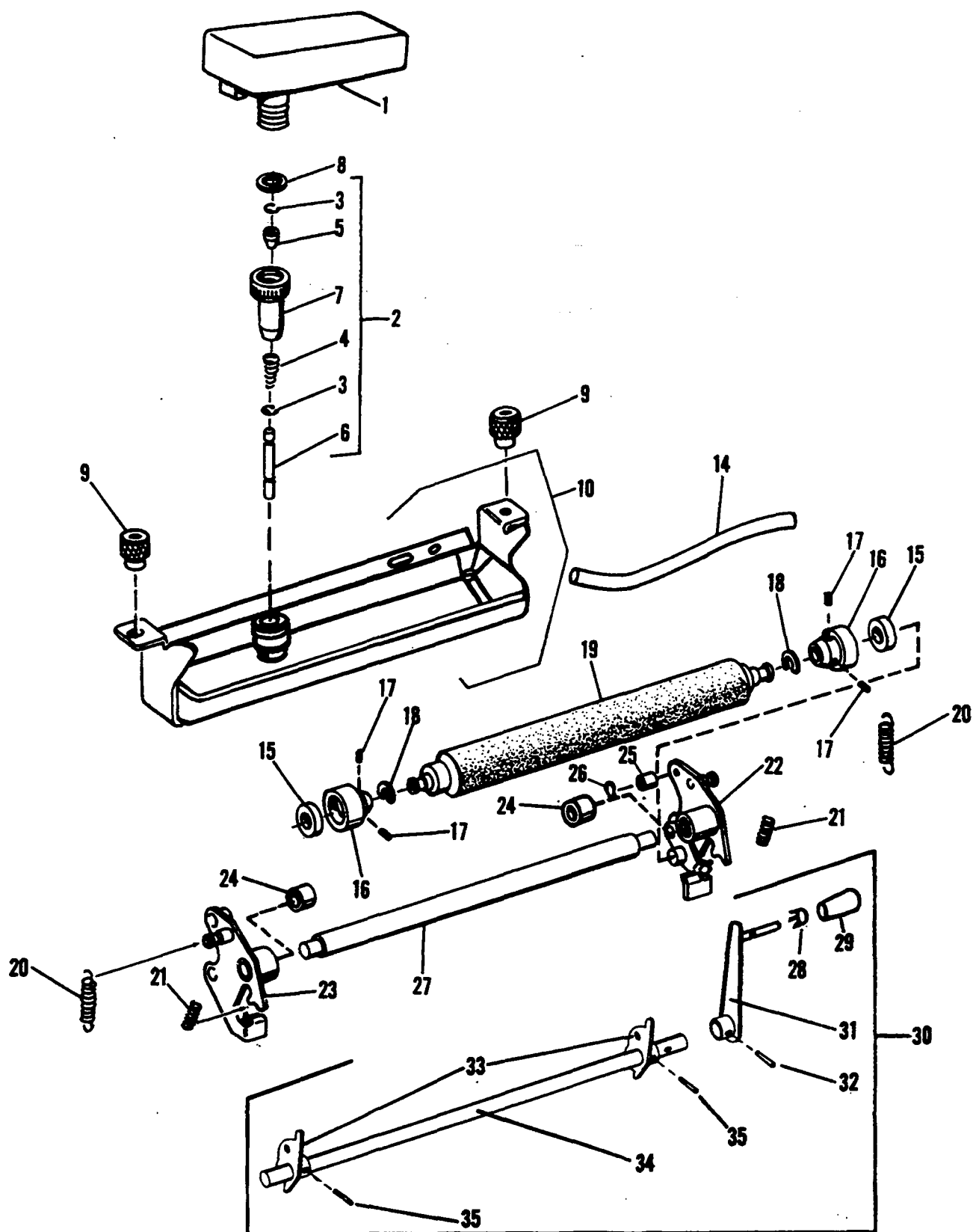
FIGURE 8 MODEL 8805/8820 Aquamatic - Part 1
