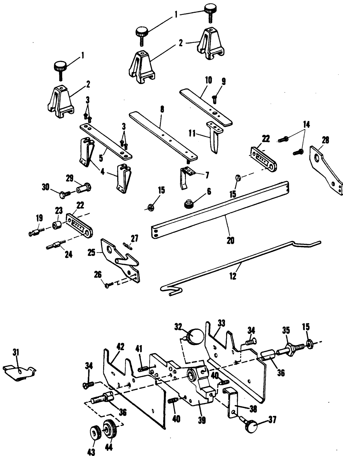
FIGURE 1 MODEL 8805/8820 Paper Guides and Mounting Bar
